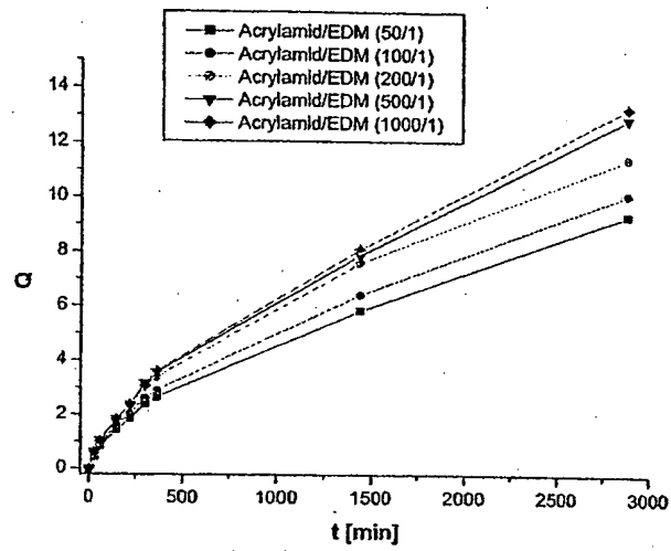
Fig. 4: Swelling experiments of acrylamide/ethylenedimethacrylate hydrogels incorporating 30 wt-% high molecular weight polyvinyl pyrrolidone (PVP)
